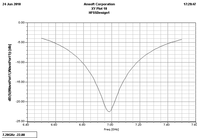
Fig.13: S11 response
