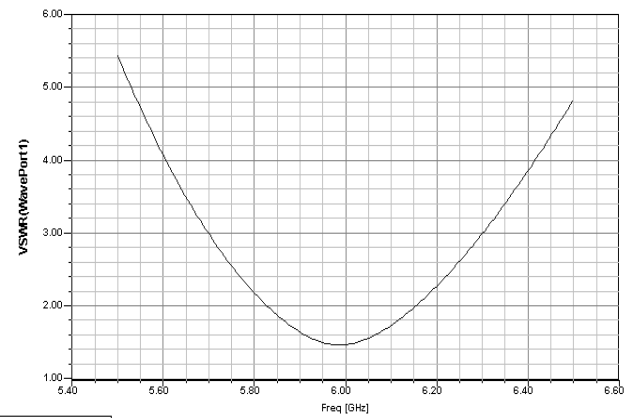
Fig.10: VSWR
