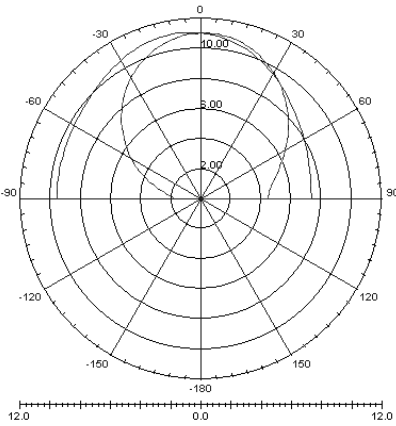
Fig.7: Radiation Pattern
