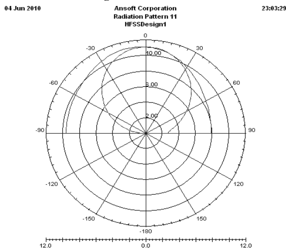
Fig.4: Radiation Pattern
