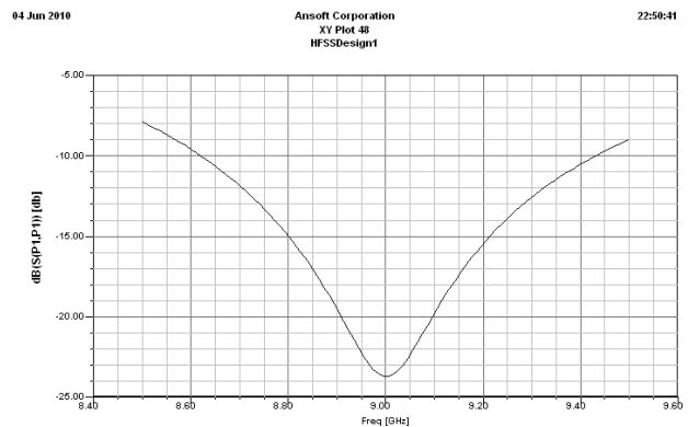
Fig.5: S11 response
