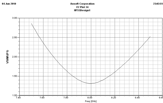
Fig.2: VSWR
