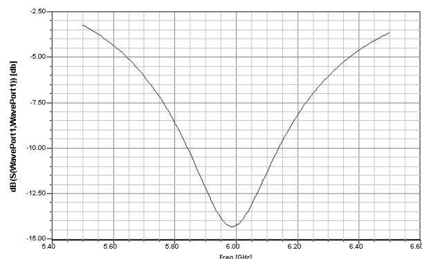
Fig. 9: S11 response
