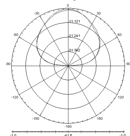
Fig.12: Antenna Gain
