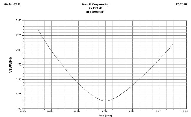
Fig.6: VSWR
