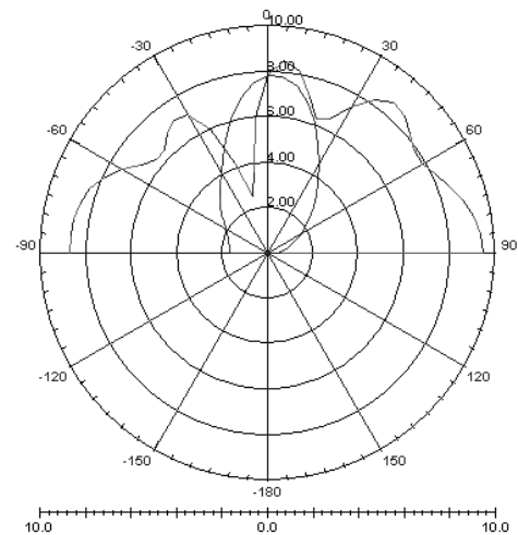
Fig.11: Radiation Pattern
